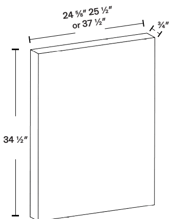
BASE END PANEL
