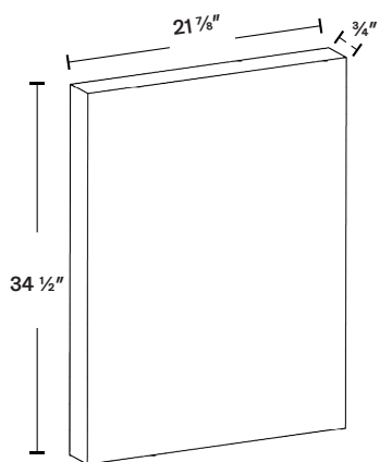
VANITY END PANEL
